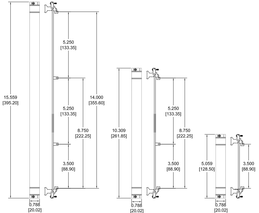
9U x 4HP
